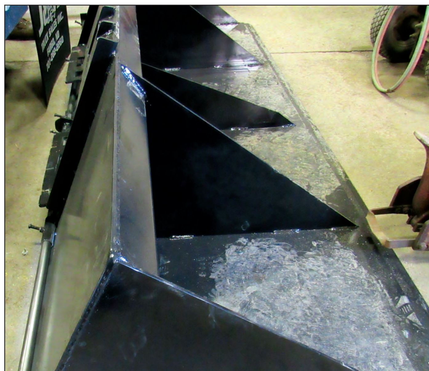
Innovation: Chip Seal Bucket Spreader
